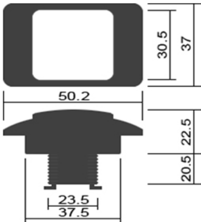
CWB 409 Button
